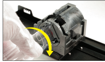
3. Rotate lamp 172° inside socket to initiate power/electrical connection
