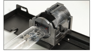
4. Lamp is now safely installed and ready for operation
